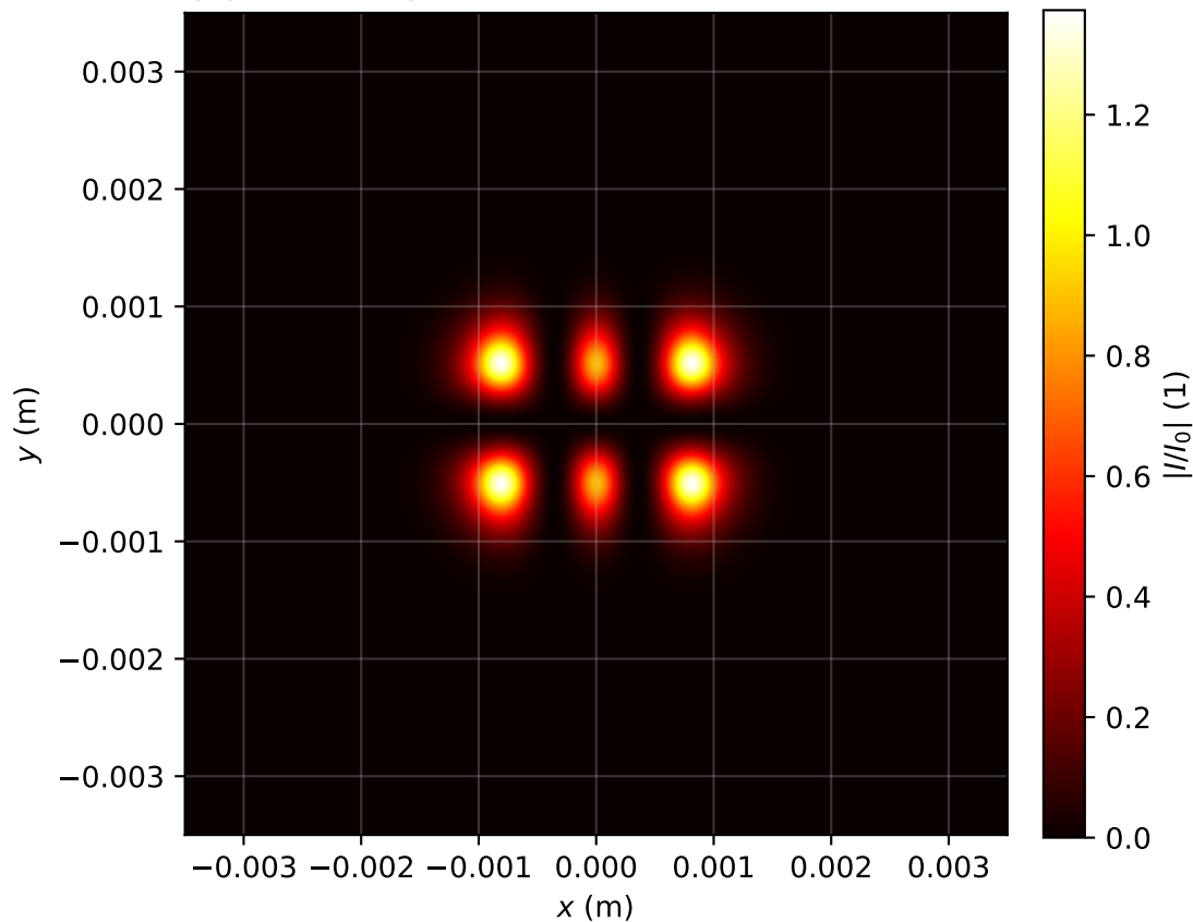
Intensity profile I(x, y, z = 0.398)/I_0 , P_{in}=3.0P_{cr} , artificial time
